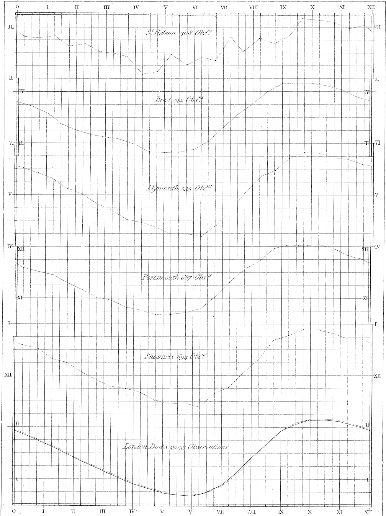
In these curves the abscissa represents the time of the Moon's transit, and the ordinate the corresponding interval between the transit & the time of High Water Observation Theory
